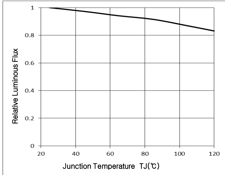
Fig 6. Junction Temperature vs. Relative Luminous Flux, I_F=65mA
