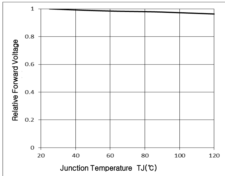
Fig 7. Junction Temperature vs. Relative Forward Voltage, I_F=65mA
